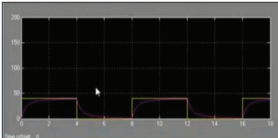
Figure 6 Steady – State response for the testing DC motor model with PI controller
