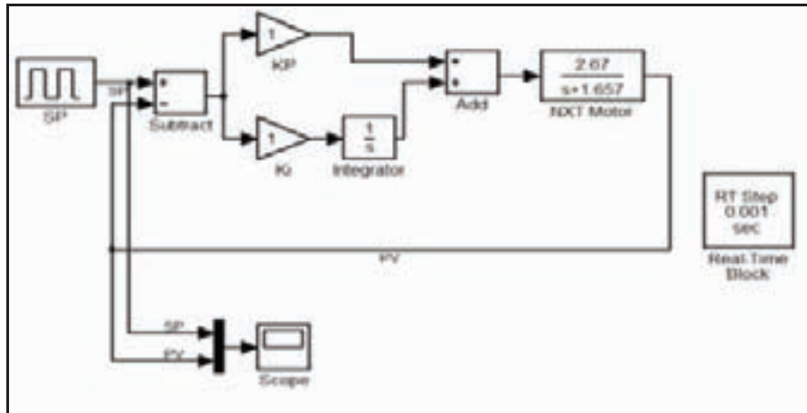
Figure 5 Block Diagram for PI controller with DC motor model
